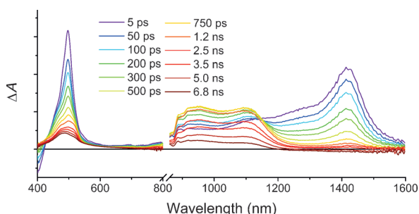
Figure 2. Combined visible and near-infrared femtosecond transient absorption spectra recorded in MeCN of ExBox 4+ , exciting at \lambda_{\text{ex}} = 330 nm ( 0.6 \mu\text{J pulse}^{-1} ), highlighting the characteristic reduced ExBIPY 2+ absorption from 900–1200 nm. Relative amplitudes on either side of the break are arbitrary.
